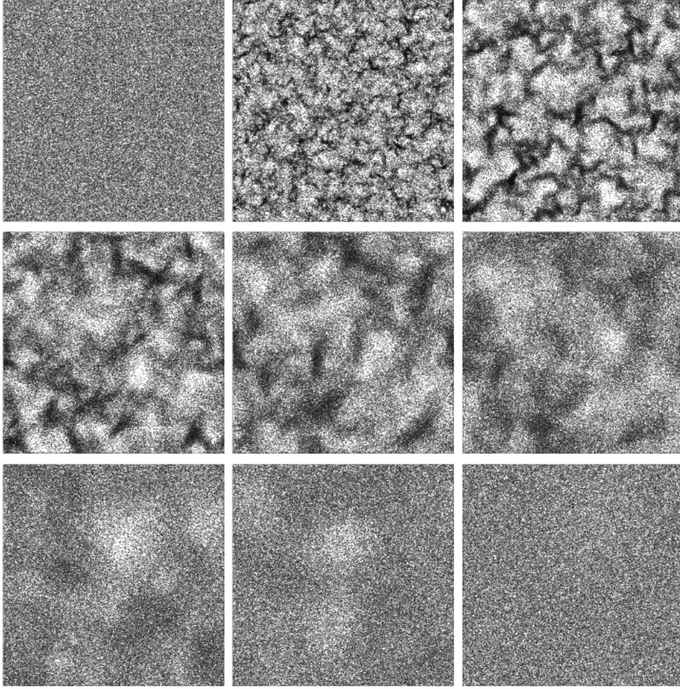
Figure 3. Snapshots of a simulation ( N = 10^5 , \varepsilon^* = 0.6 , g^* = 0.1 , \eta = 0.1 ) after 0, 50, 100 (first row), 150, 200, 250 (second row), 500, 1000 and 5000 (last row) collisions per particle. The corresponding fractions of dissipatively occurring collisions read (in the same order) 0.998, 6 \times 10^{-3} , 1.1 \times 10^{-3} , 5.1 \times 10^{-4} , 3 \times 10^{-4} , 2.8 \times 10^{-4} , 8.5 \times 10^{-5} , 2.6 \times 10^{-5} , 3.8 \times 10^{-6} . The initial temperature T_0 = 1 corresponds to the thermal velocity v_T = \sqrt{2} . Starting at a homogeneous distribution we observe cluster formation up to a certain cluster size. At late times the system returns to the homogeneous cooling state.
