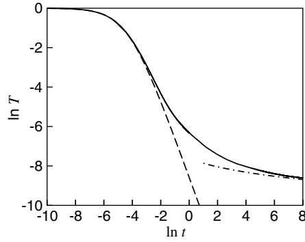
Figure 2. Granular temperature of a gas of N = 10^5 particles and critical velocity g^* = 0.1 . Full curve: molecular dynamics, dashed curve: Haff's law, equation (5), dash-dotted curve: asymptotics, equation (21).
