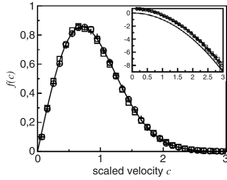
Figure 1. Scaled velocity distribution f(c) at times t_1 < t_2 < t_3 where v_T(t_1) \gg g^* (circles), v_T(t_2) \approx g^* (squares) and v_T(t_3) \ll g^* (plus symbols), together with a Maxwellian (full curve). Inset: the same data as \ln(f(c)/c) . The full curve shows a parabola for comparison (shifted for better visibility).
